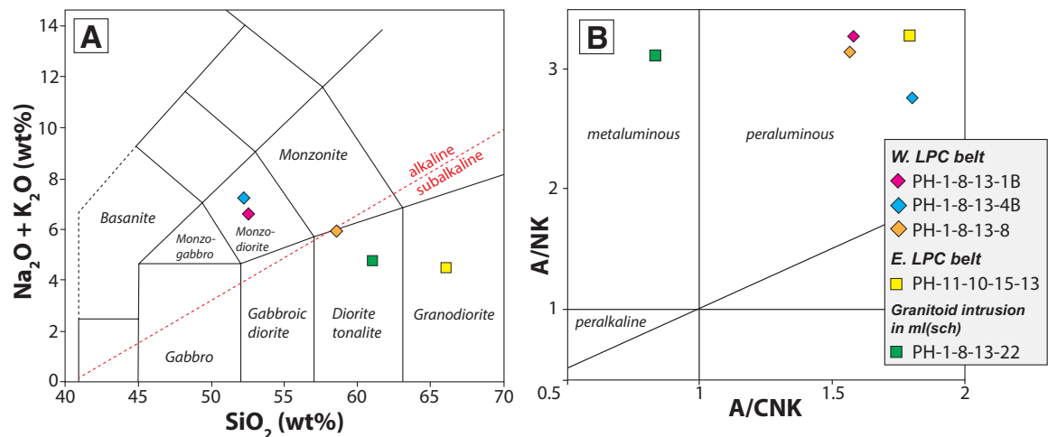
Figure 12. Geochemical plots for plutonic rocks including (A) alkalis versus silica classification and (B) Al_2O_3/N_2O + K_2O versus Al_2O_3/CaO + N_2O + K_2O . Plots are based on the methods of Shand (1943) and Le Bas et al. (1986). LPC—Lohit Plutonic Complex.
